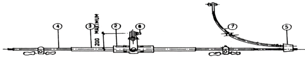
OPGW SUSPENSION — FITTINGS
